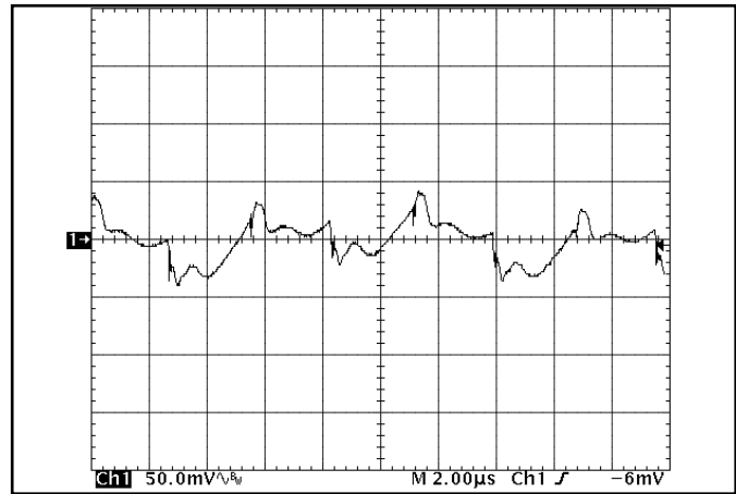
Figure 20: Output voltage ripple at nominal input voltage and rated load current (50 mV/div). Load capacitance: 1\ \mu\text{F} ceramic capacitor and 15\ \mu\text{F} tantalum capacitor. Bandwidth: 500 MHz. See Figure 17.
