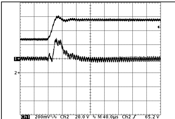
Figure 21: Output voltage response to step-change in input voltage (50V to 100V in 40\ \mu\text{s} ). Load cap: 10\ \mu\text{F} , 100\ \text{m}\Omega ESR tantalum capacitor and 1\ \mu\text{F} ceramic cap. Ch 1: V_{\text{out}} (200mV/div), Ch 2: V_{\text{in}} (20V/div).
